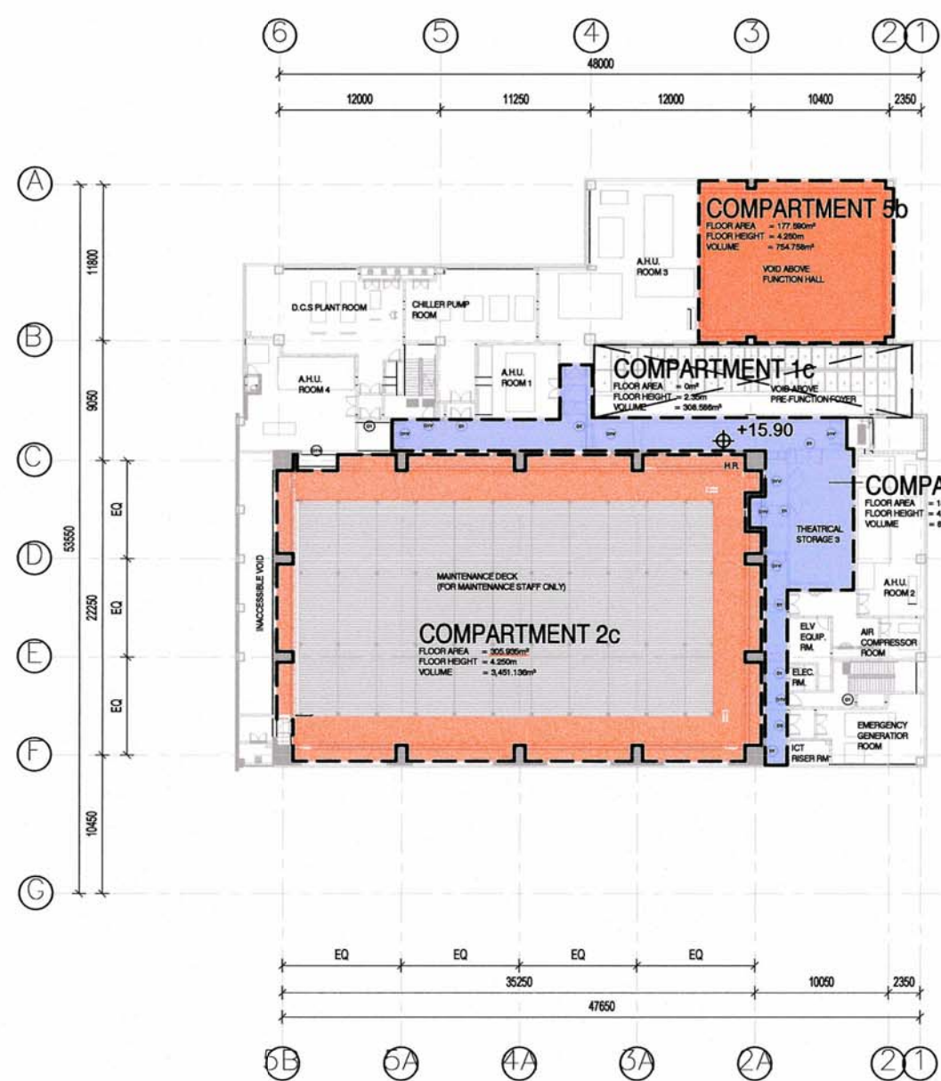
2/F COMPARTMENTATION DIAGRAM
