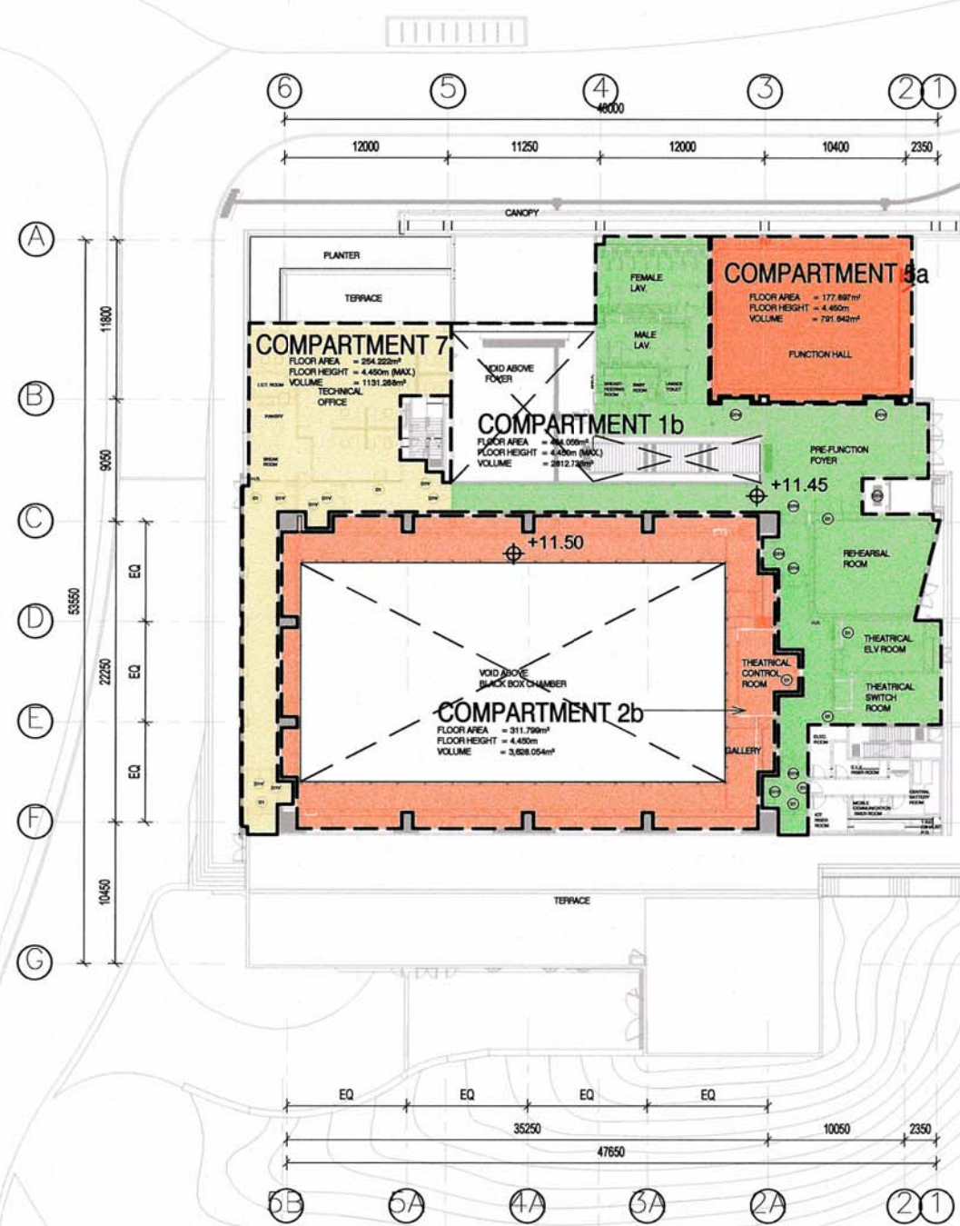
1/F COMPARTMENTATION DIAGRAM
