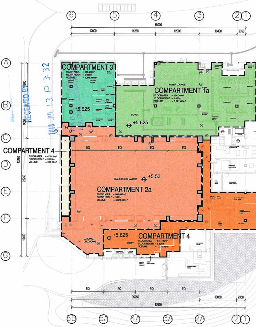
G/F COMPARTMENTATION DIAGRAM
